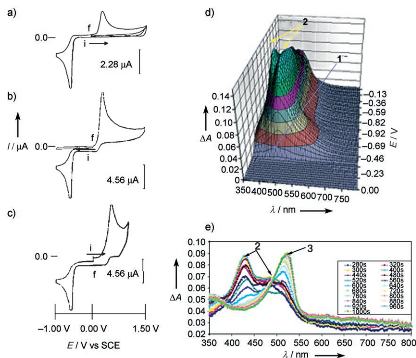
Figure 1. Cyclic voltammetry (CV) at 4.0 mM in \text{CH}_3\text{CN} with 0.1 M n\text{Bu}_4\text{NBF}_4 at 10^\circ\text{C} . Scan rate 1.0\text{ V s}^{-1} , glassy carbon disk electrode (0.05 mm diameter). a) 1 in the potential range 0.00/1.50/−1.00/0.00 V (two cycles). b) 2 in the potential range 0.00/−1.00/1.50/0.00 V (two cycles). c) 3 in the potential range 0.00/1.00/−1.00/0.00 V. d) Spectroelectrochemical scan of 1 (0.5 mM) with scan rate 0.1\text{ V s}^{-1} in the potential range 0.00/−1.00/0.00 V; 60 spectra were recorded during the scan. [15] e) In situ UV/Vis spectra during electrolysis of 1 (0.5 mM) at −1.00 V vs. Ag/AgCl in a spectroelectrochemical cell with Pt minigrid as working electrode. [15]
